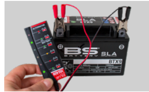
BT02 - BATTERY & ALTERNATOR TESTER
